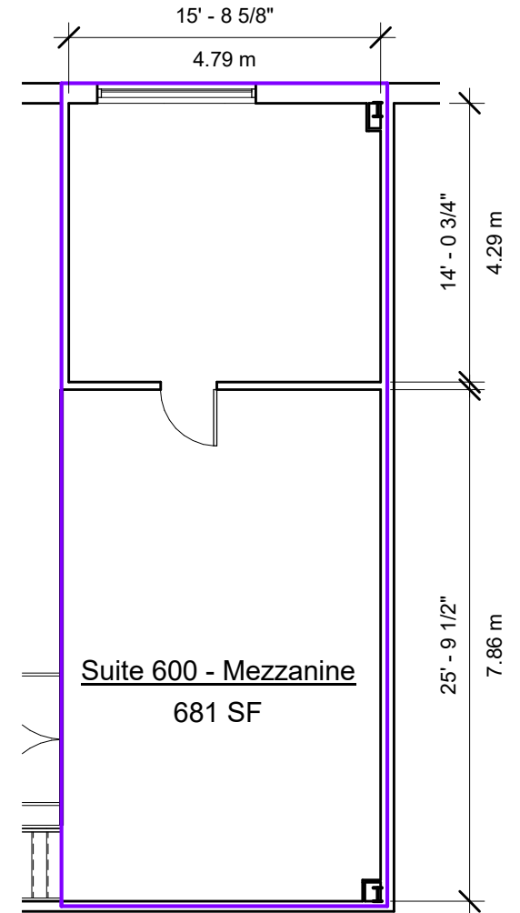
③ Suite 600 - Mezzanine 1/8" = 1'-0"
