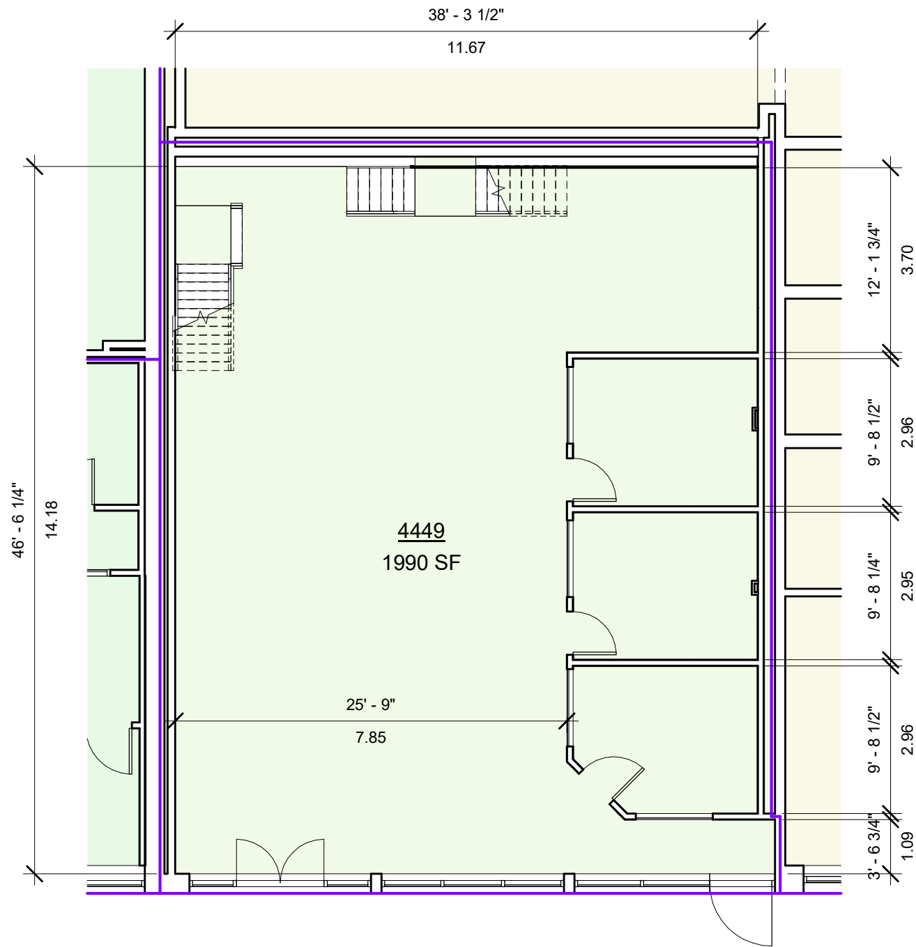
① 4449 - RDC 1/8" = 1'-0"
